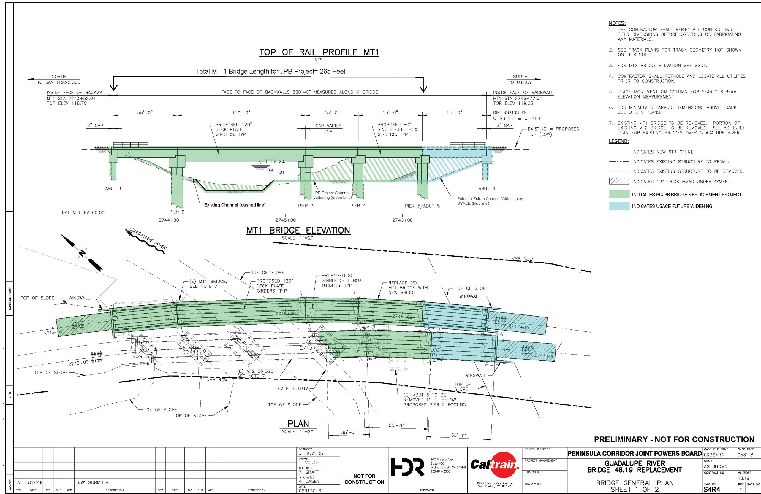
Figure 2. Project 35 Percent Design Plans (1 of 2).
