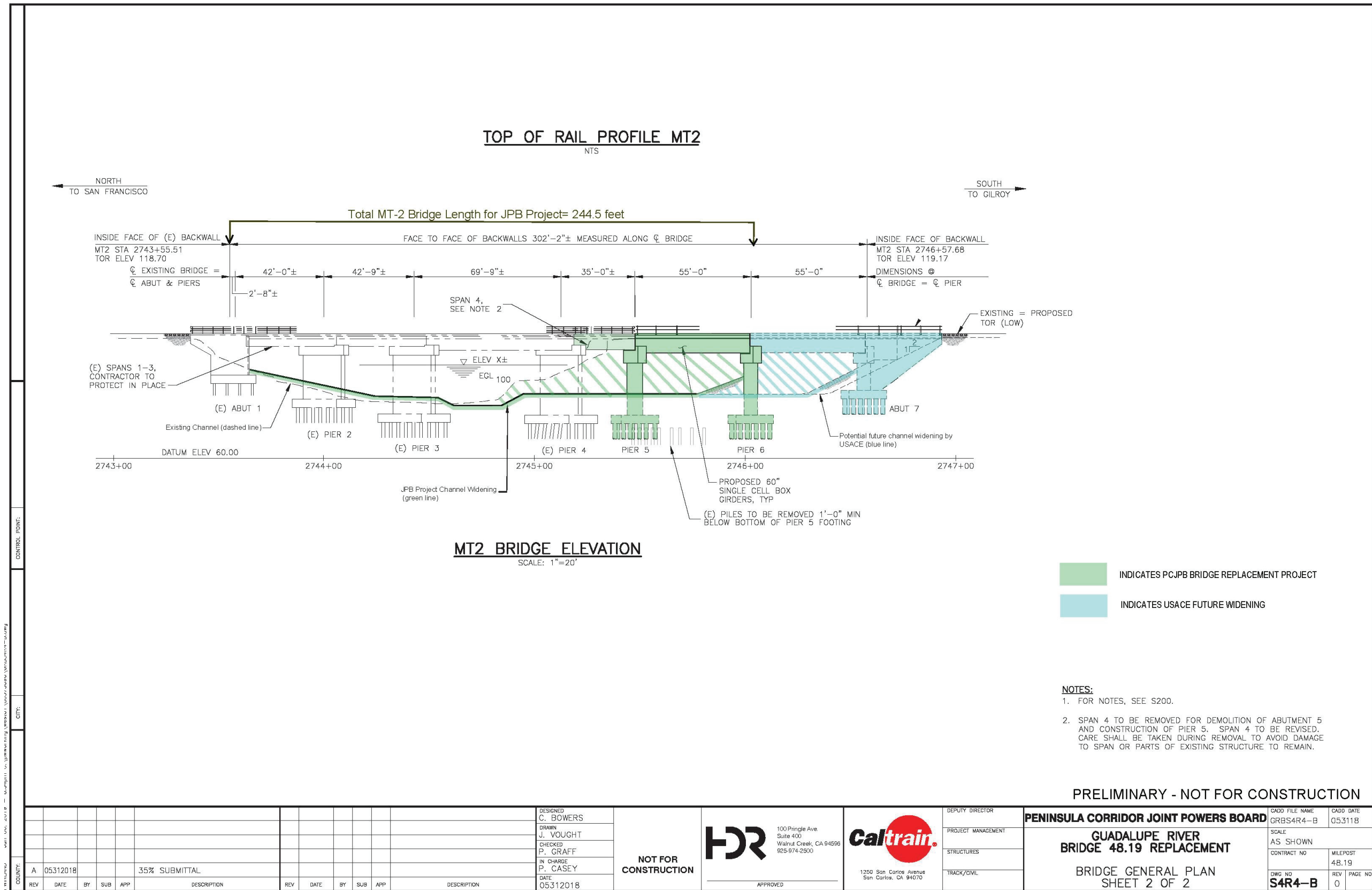
Figure 2. Project 35 Percent Design Plans (2 of 2).
