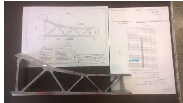
Carbody - Aluminium Section of End Underframe
