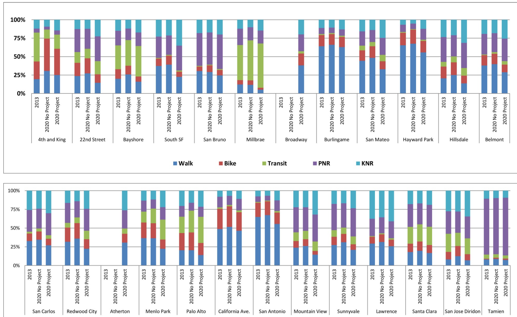
Figure 3-21 AM Modes of Access, 2020 No Project and Project Scenarios
