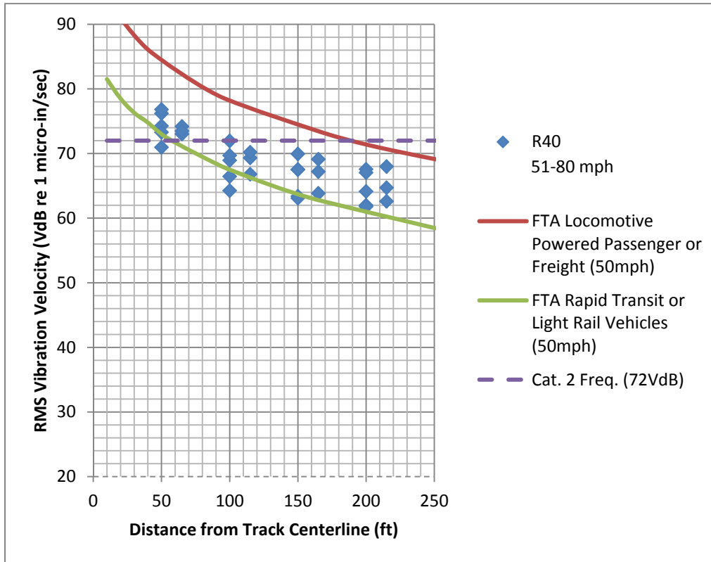
Figure B-7 Measured at Site R40 on Wednesday, June 5, 2013 Vibration data shown has not been normalized to 50 mph.
